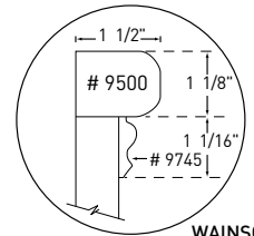
WAINSCOT CAP MOULDINGS SECTION AA
