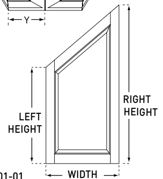
90-8150-01-01 Special application angled door
