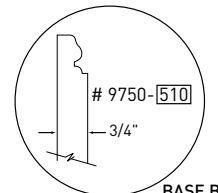
BASE BOARD SECTION BB
