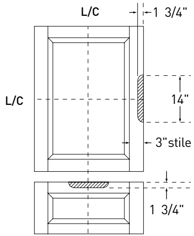
Option 534 (on stile)
