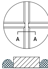
SECTION AA Mullions with added beads.
