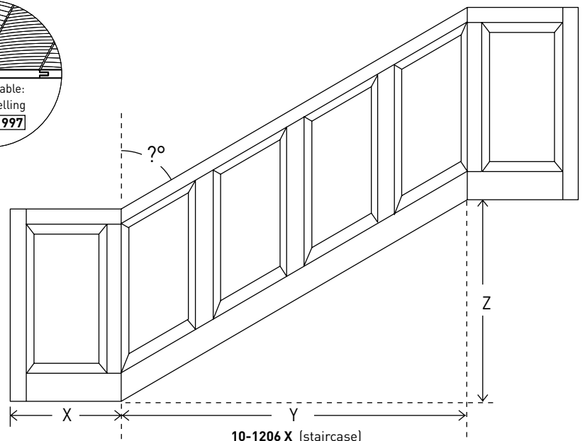
10-1206 X (staircase)
